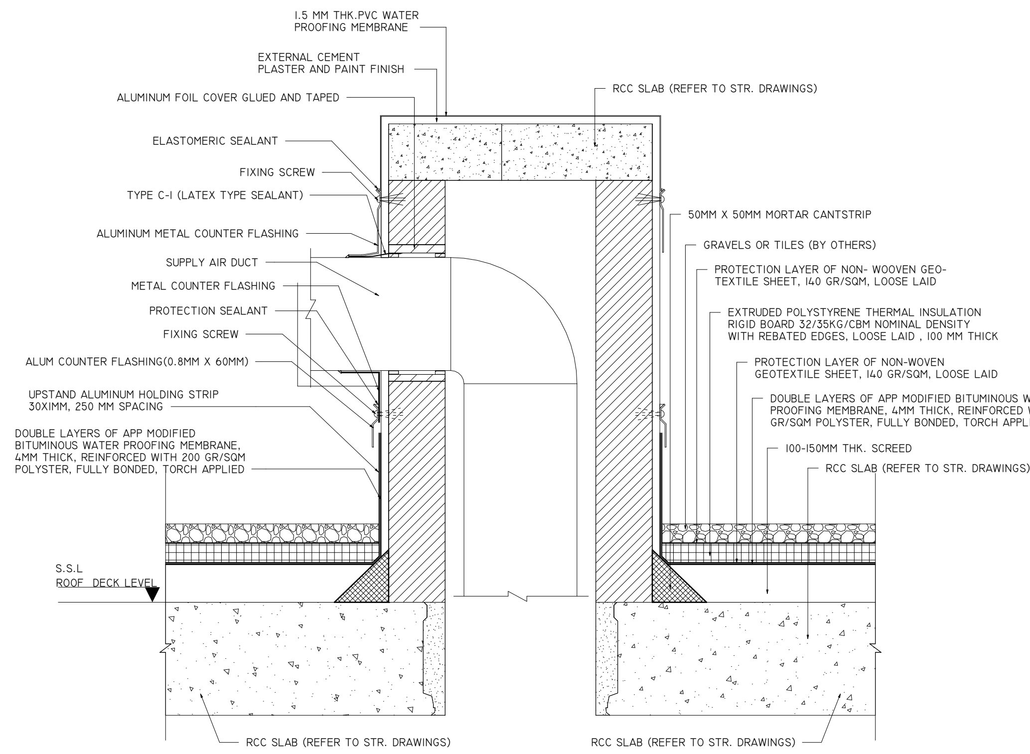
1 TYPICAL AIR DUCT - THROUGH ROOF 1 : 10
