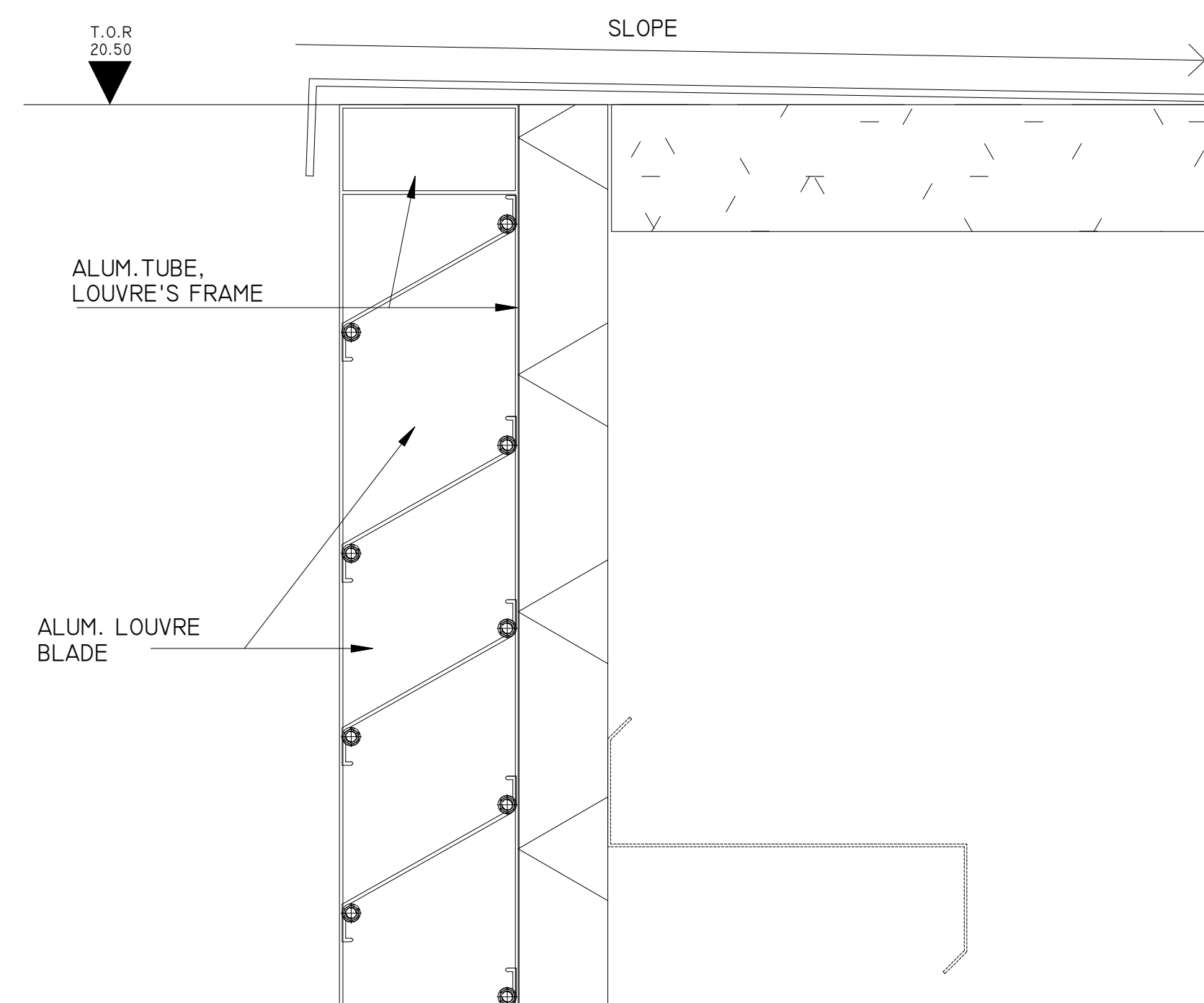
5 FLASHING DETAILS AT PARAPET 1 : 5
