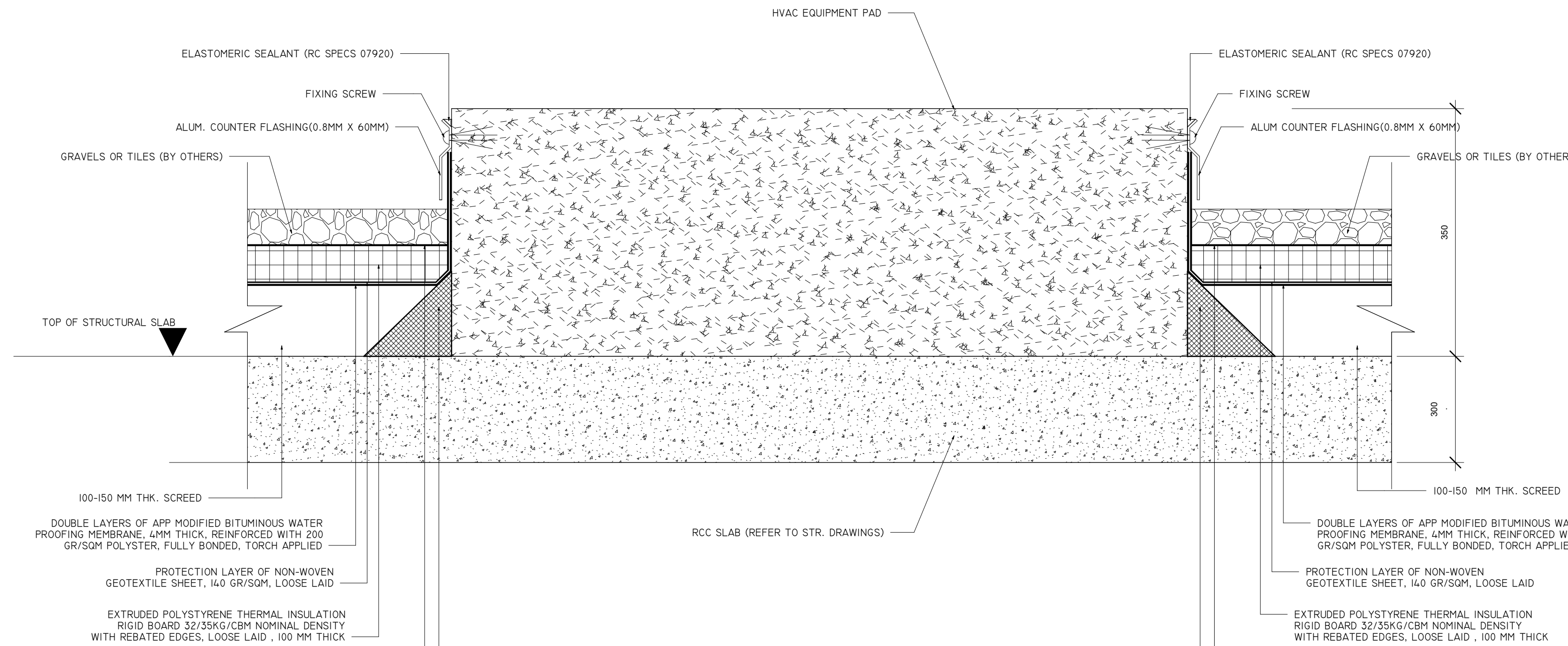
2 TYPICAL HVAC QEQUIPMENT PAD DETAIL 1 : 5
