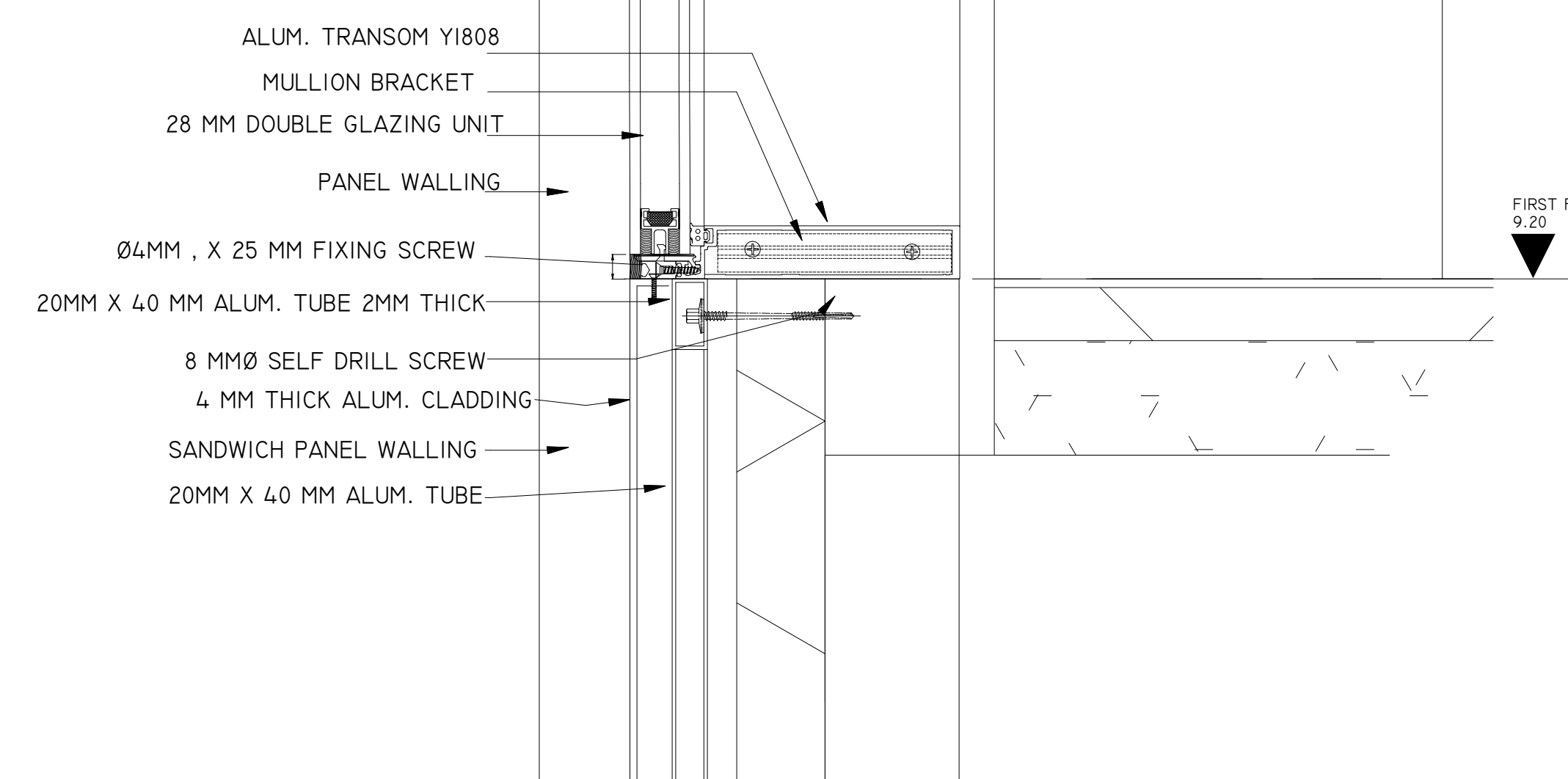
7 CURTAIN WALL CONNECTION ON SLAB DETAILS 1 : 5
