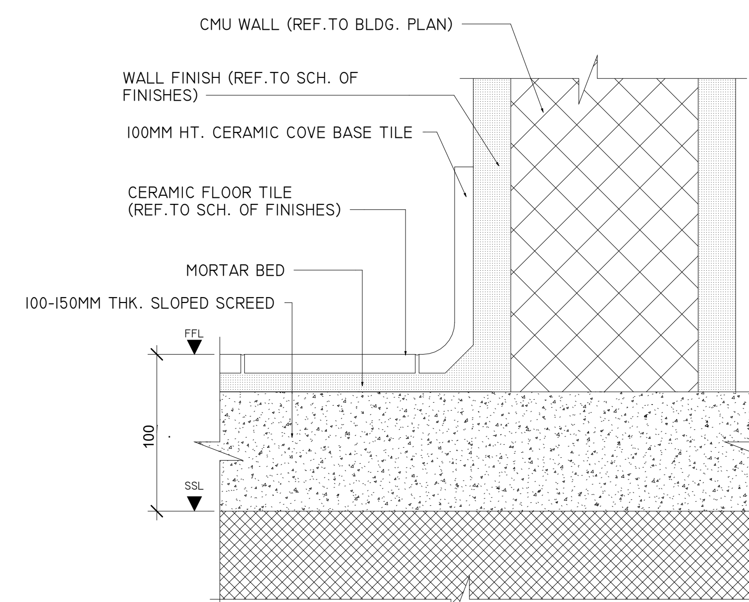
9 CERAMIC TO CERAMIC DETAIL 1 : 2
