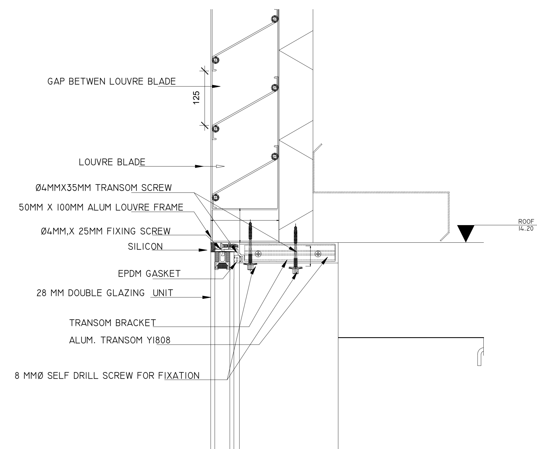
4 LOUVER TO CURTAIN WALL DETAILS 1 : 5
