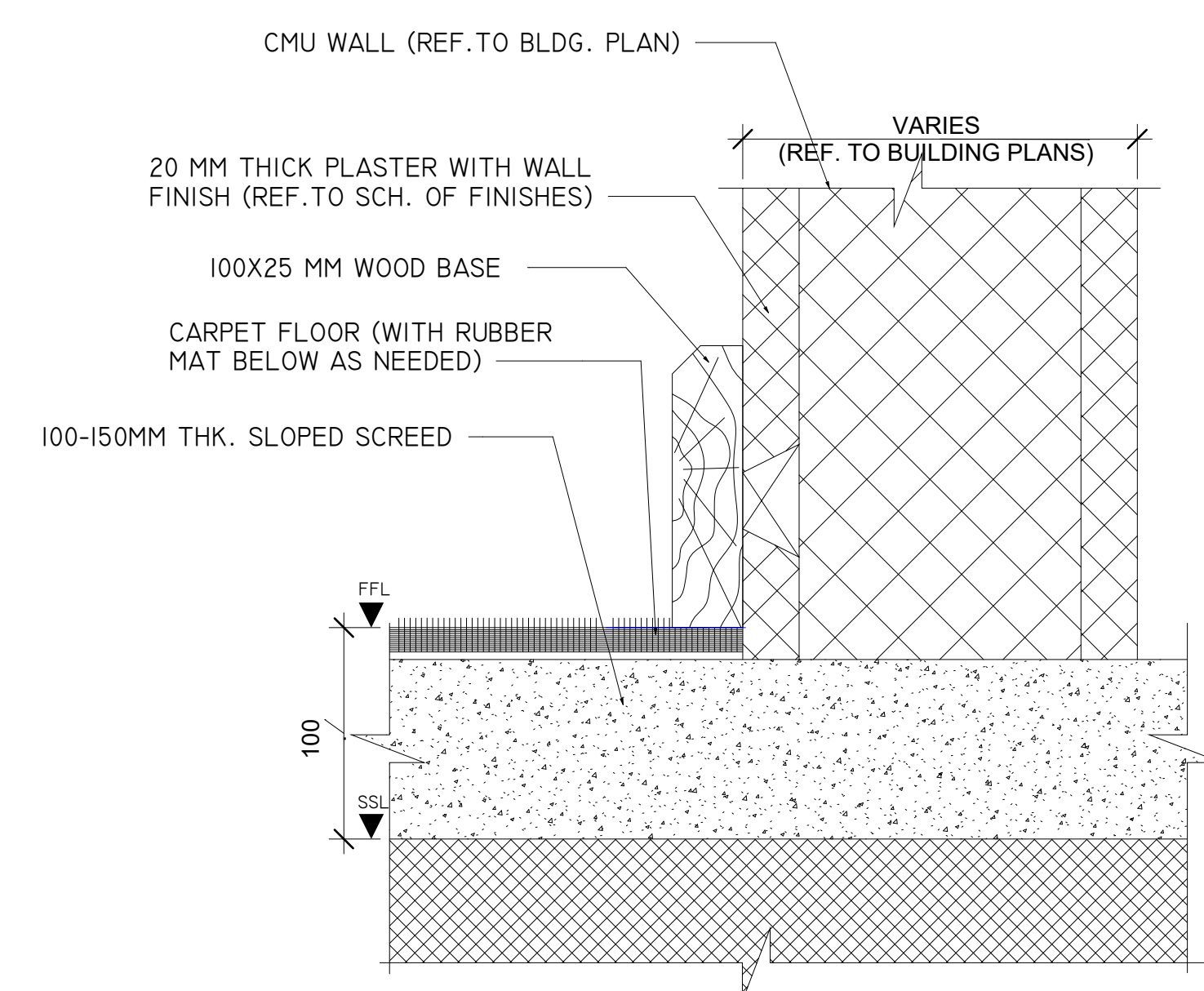
8 CARPET TO WOOD DETAIL 1 : 2
