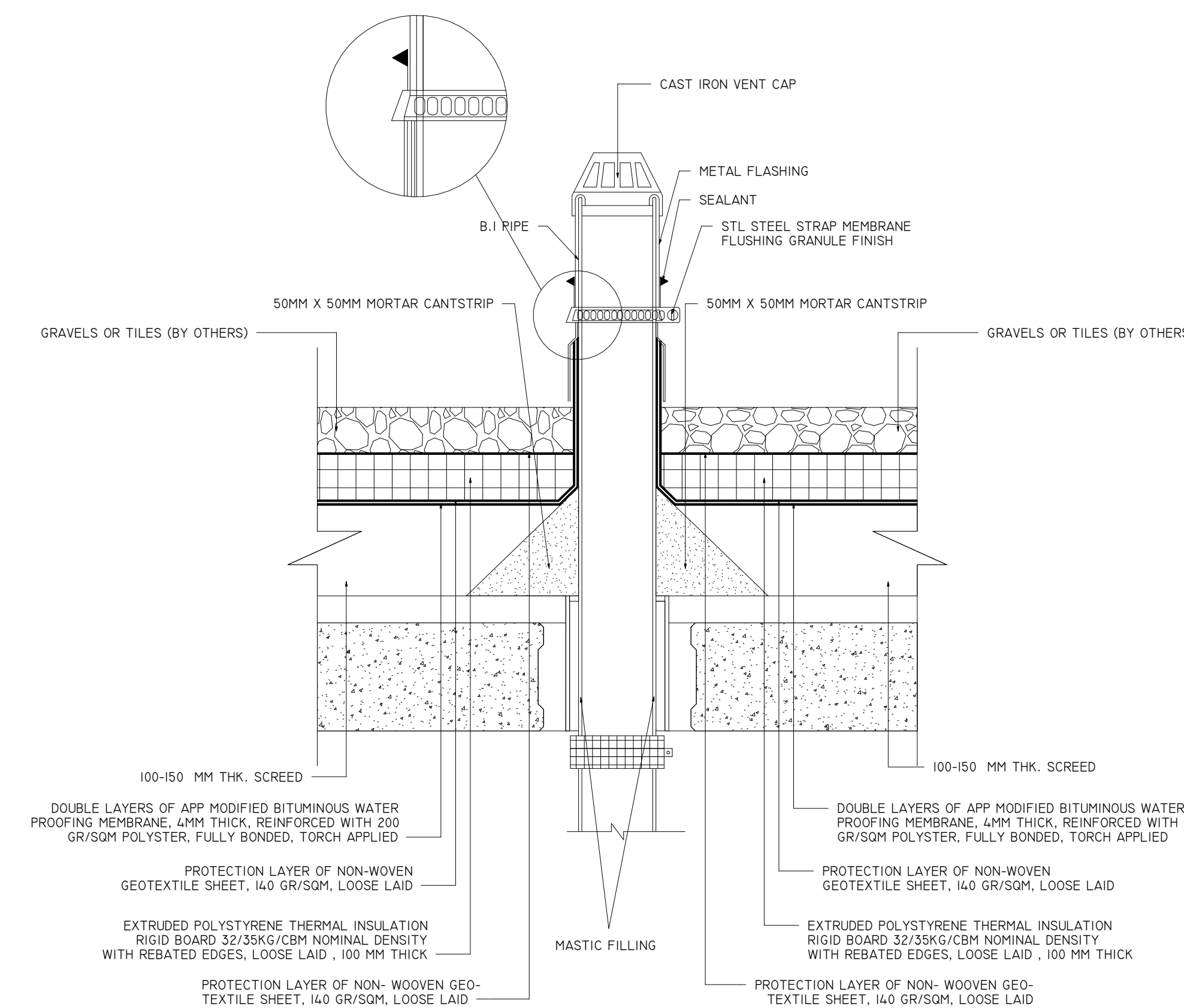
3 TYPICAL VENT THROUGH ROOF DETAIL 1 : 5
