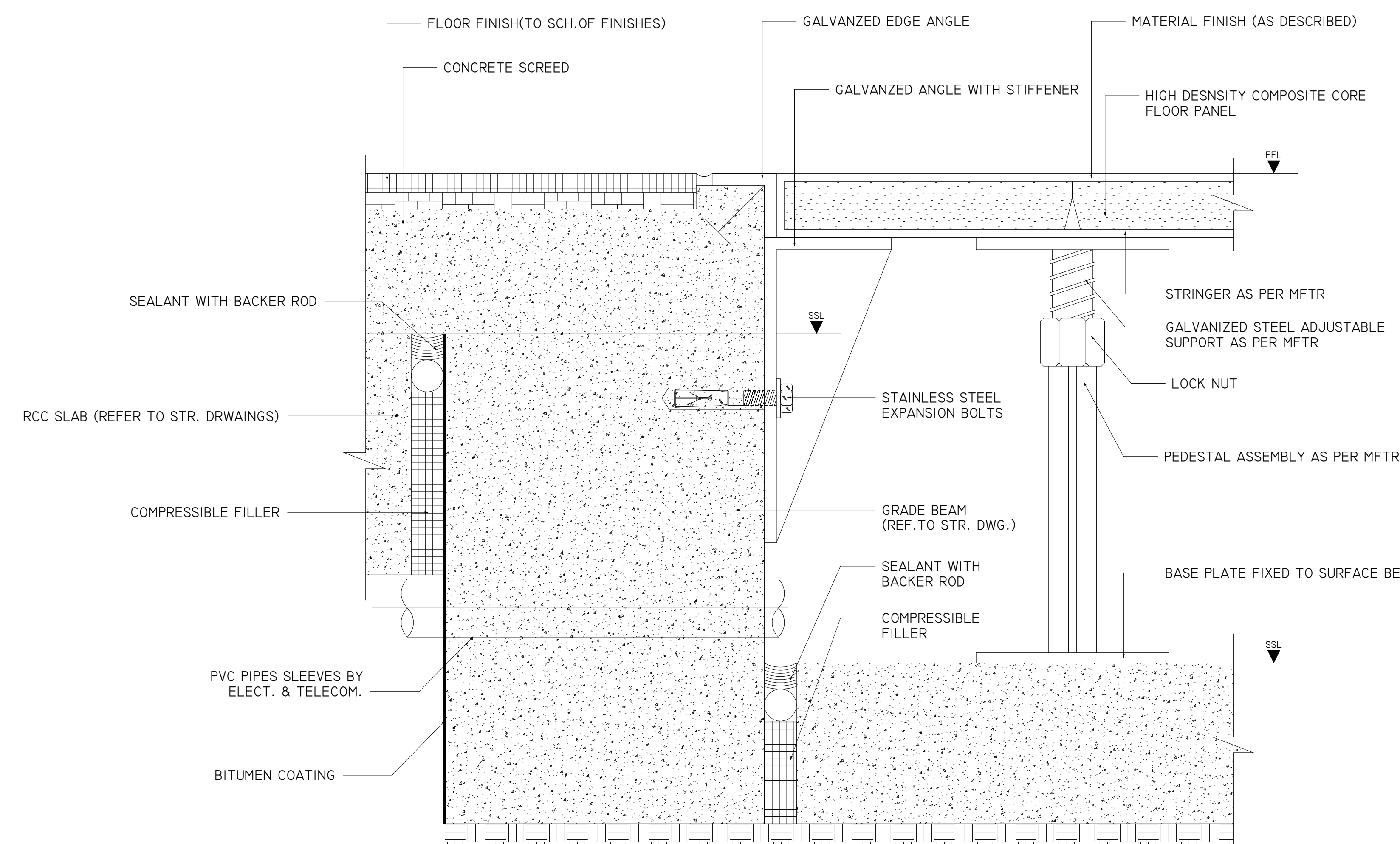
10 RAISED FLOOR DETAIL (INTERNAL) 1 : 2
